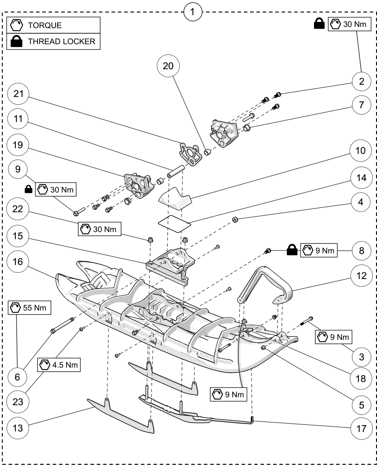
SKI ASSEMBLY
