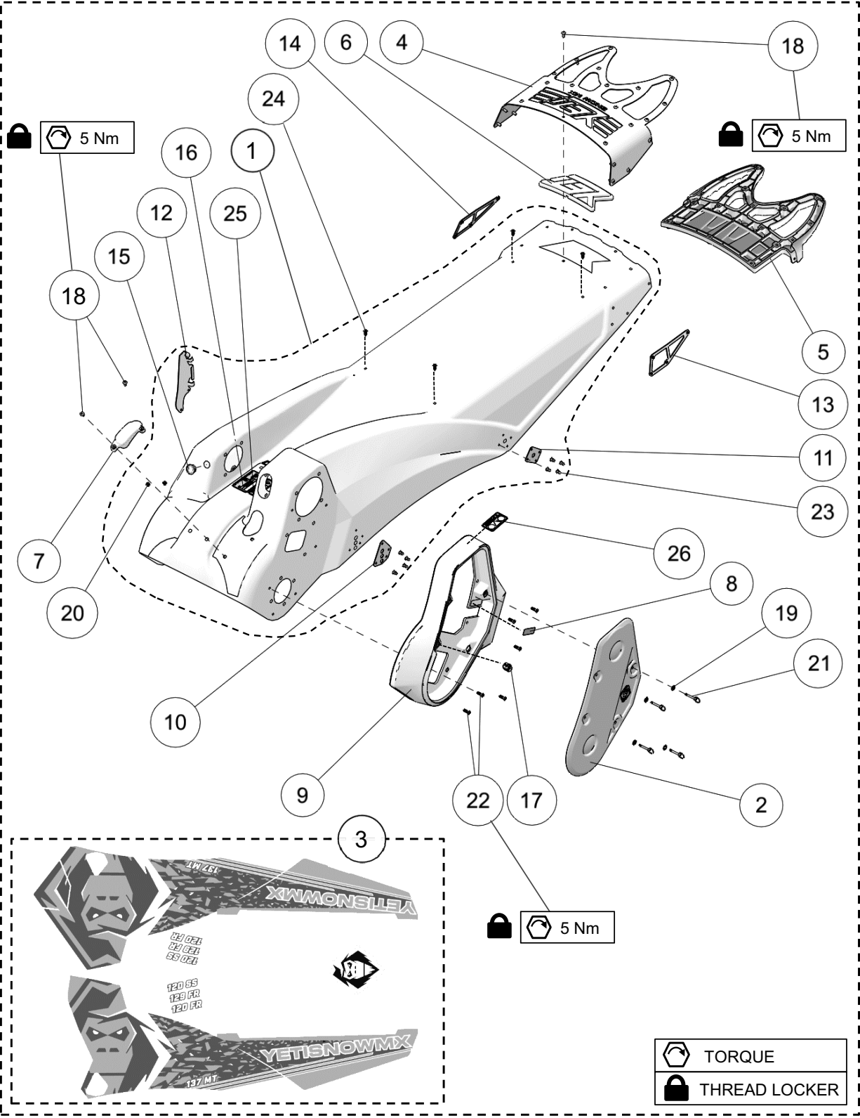
CHASSIS ASSEMBLY - 120FR - 129FR - 137MT
