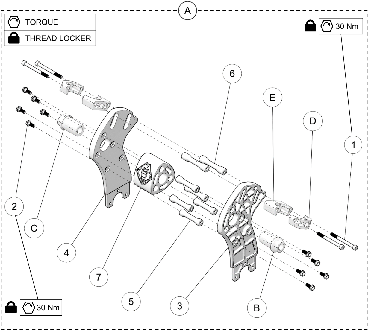
SPINDLE ASSEMBLY
