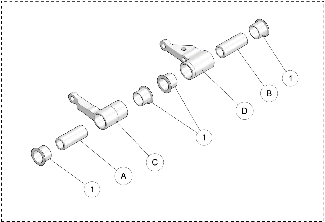
BIKE MOUNT ADAPTER ASSEMBLY
