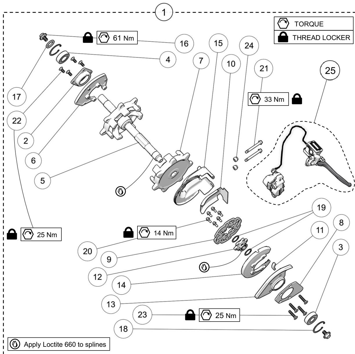
DRIVE SHAFT ASSEMBLY - YETI 129FR &amp; 137MT
