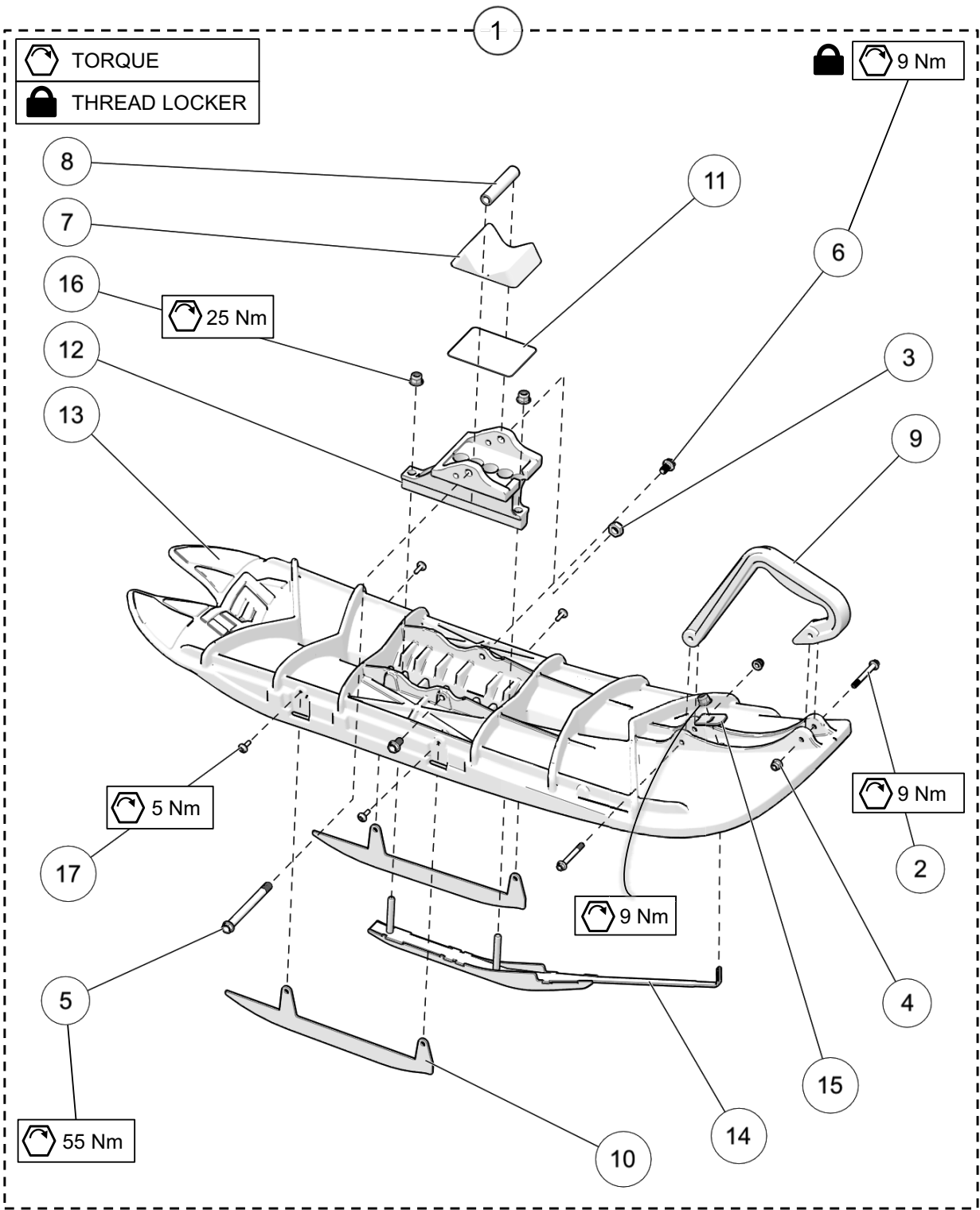
SKI ASSEMBLY
