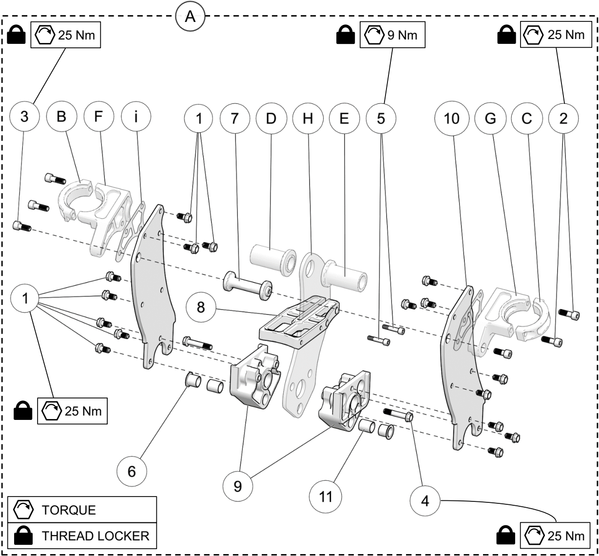
SPINDLE ASSEMBLY
