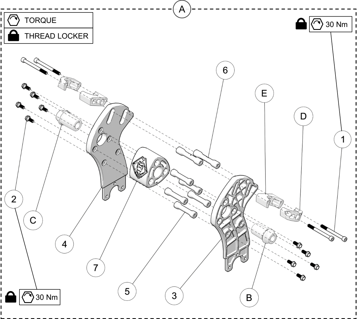
SPINDLE ASSEMBLY
