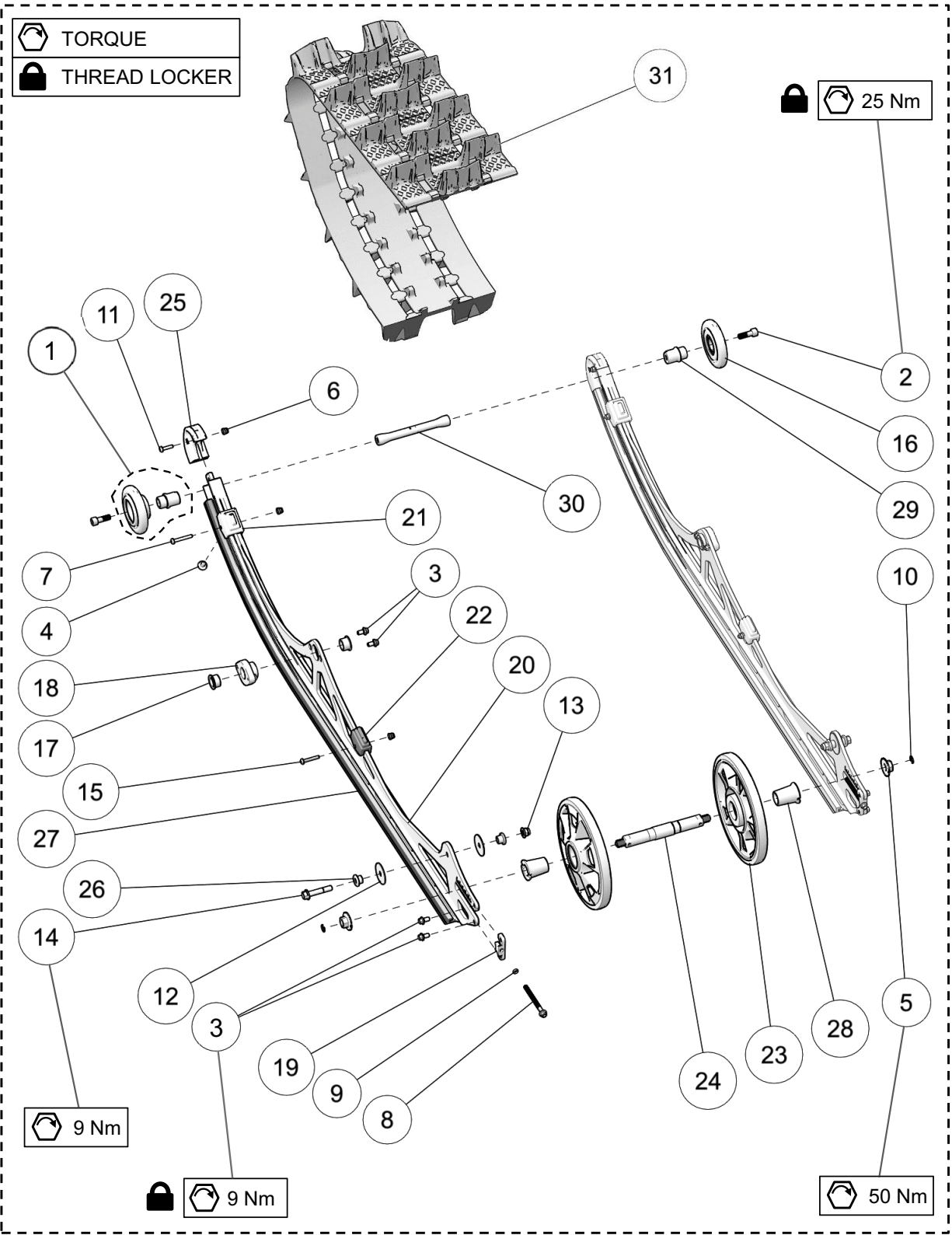
RAIL ASSEMBLY, TRACK - YETI 120FR / 129FR / 137MT
